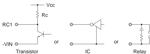
Fig.4.2 RC1 connection example
